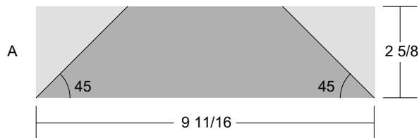
Cutting Diagrams
